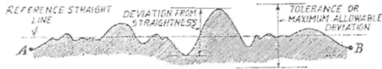
Fig. 1: Profile of surface with respect to reference straight line.
